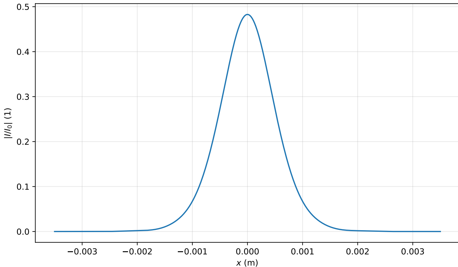
Intensity profile I(x, y = 0, z = 3.981m)/I_0 , P_{in}=0.6P_{cr} , artificial time
